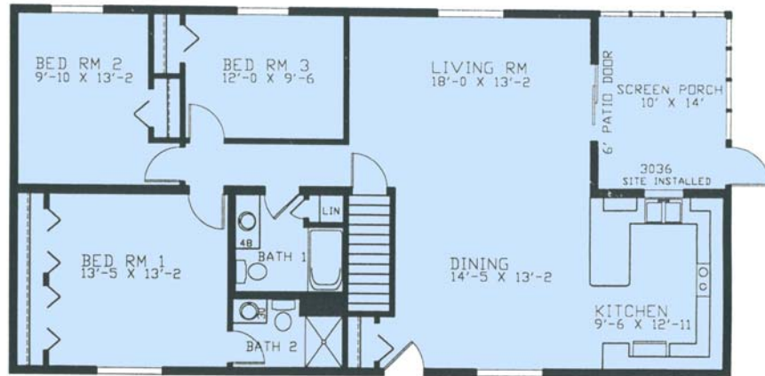
Design V109 Size 54' x 28' Area 1372 sq. ft.
