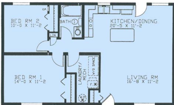
Design V104 Size 40' x 24' Area 960 sq. ft.
