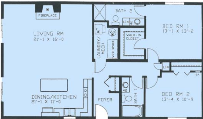
Design V101 Size 48' x 28' Area 1344 sq. ft.
